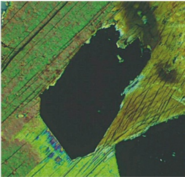
Feldspar crystal, linear polarized light, dark setting
