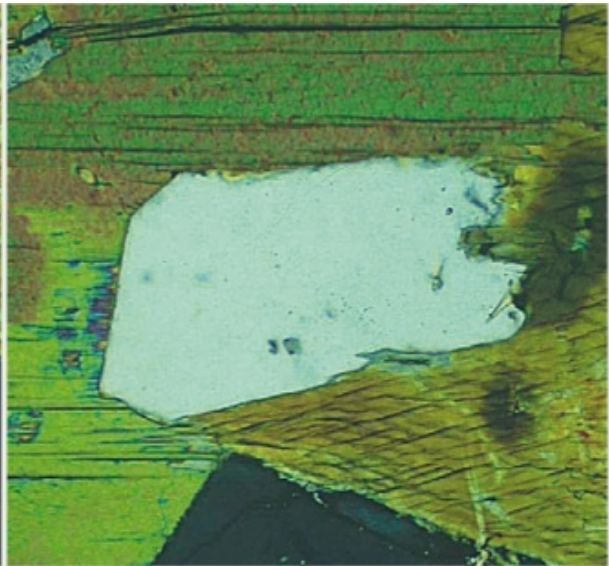
Feldspar crystal, linear polarized light, light setting
